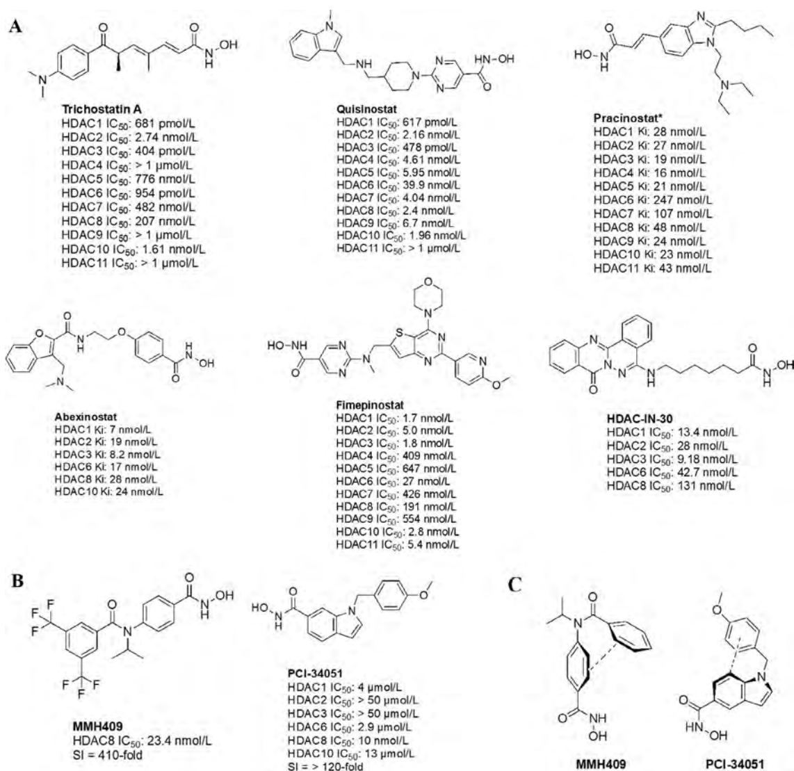
Figure 6. Pan-HDACi overview. (A) Broadly acting pan-HDACs bearing a hydroxamate ZBG that exhibit target engagement towards class I HDACs; (B) inhibitors bearing a hydroxamate ZBG that are HDAC8-selective [42–49]; (C) potential “ cis ” conformations adopted by HDAC8-selective inhibitors [43]. * Asterisks refer to inhibitors that are either clinical candidates or FDA-approved drugs. SI: selectivity index; Ki: inhibition constant
