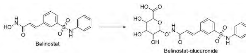
Figure 13. Overview of the chemical reaction of belinostat transformation. Transformation of belinostat to belinostat glucuronide in phase II metabolism [75–77]
