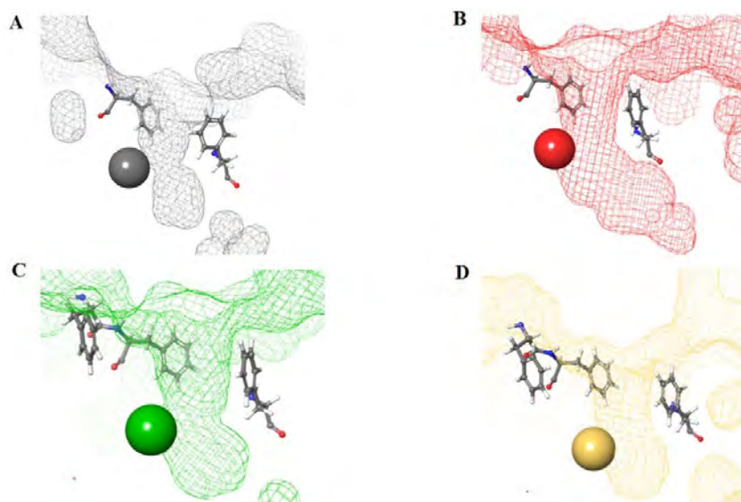
Figure 8. Structural presentation of class I HDAC catalytic centers. Class I HDAC tunnels surrounded by hydrophobic Phe residues. (A) HDAC1 (grey mesh) surrounded by Phe150 (in front of the tunnel in the image) and Phe205 (behind the tunnel in the image); (B) HDAC2 (red mesh) surrounded by Phe155 (in front of the tunnel in the image) and Phe210 (behind the tunnel in the image); (C) HDAC3 (green mesh) surrounded by Phe144 (in front of the tunnel in the image) and Phe199 and Phe200 (behind and to the side of the tunnel in the image); (D) HDAC8 (gold mesh) surrounded by Phe152 (in front of the tunnel in the image), Phe207, and Phe208 (behind and to the side of the tunnel in the image). All images in this figure were generated by Maestro
