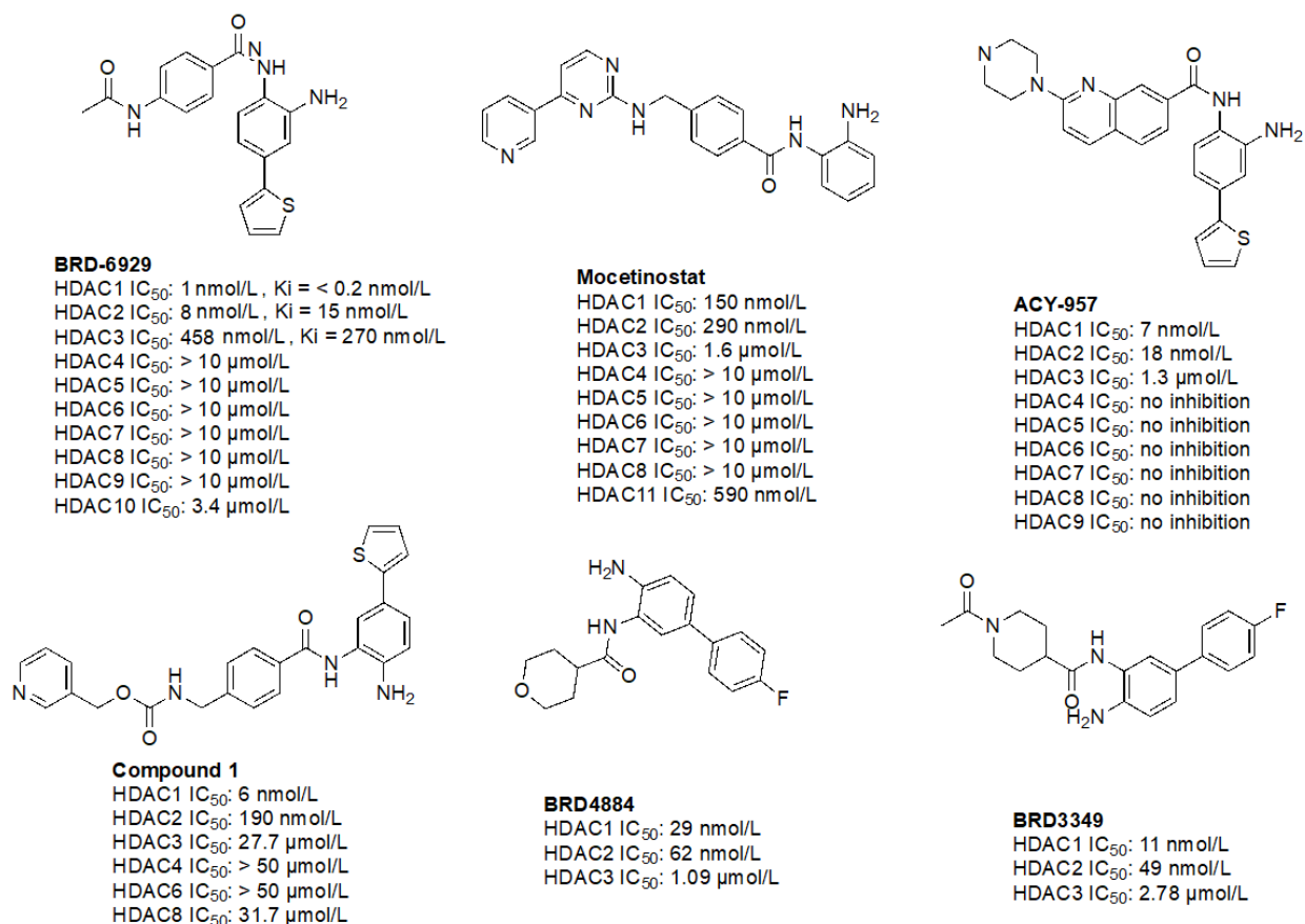
Figure 10. Examples of selective HDAC1/2 inhibitors [55, 60–64]
