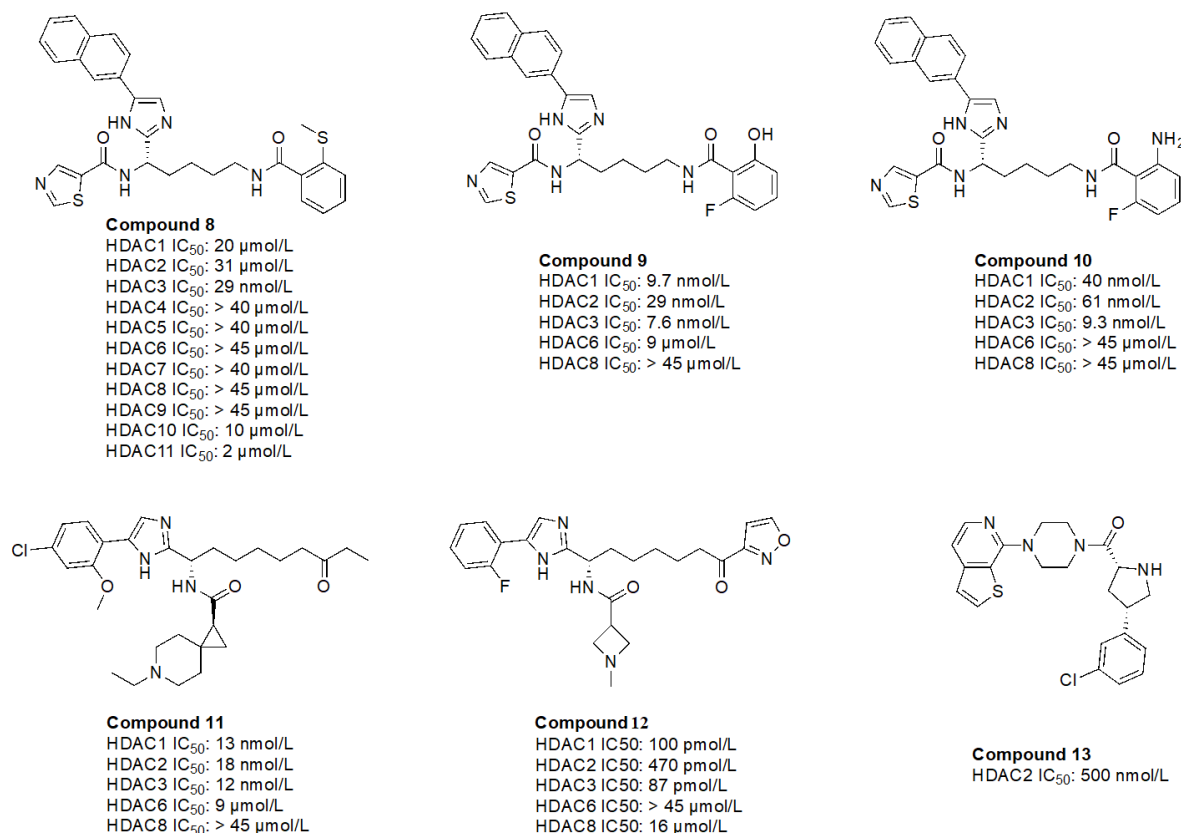
Figure 16. Examples of recently discovered novel ZBGs [88–91]
