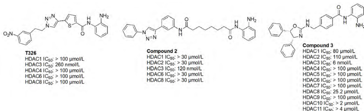
Figure 12. Examples of HDAC3 selective inhibitors [72–74]
