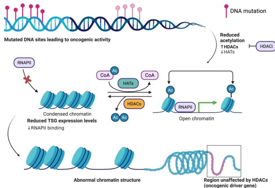
Figure 1. The basic principle of acetylation status for open (euchromatin) or closed chromatin (heterochromatin). Structural organization of DNA wrapped around histone proteins, and the effects on expression of proteins such as TSG transcription due to the downregulation of HATs and upregulation of HDACs during oncogenic activity in the cell. Acetylation of histones on surface exposed Lys residues by HAT. Histone acetylation yields an amide that is neutral at physiological pH and thus weakly interacts with the negatively charged DNA, thus allowing the cellular transcription machinery to access TSGs for transcription. Deacetylation of histones by HDAC. Histone deacetylation yields a primary amine that is positively charged at physiological pH and thus strongly interacts with the negatively charged DNA, thus preventing the cellular transcription machinery (ie. RNAPII) from accessing TSGs for transcription. HDACi aid in the inhibition of HDAC activity. The figure was created with Biorender.com . RNAPII: RNA polymerase II; CoA: coenzyme A; Ac: acetyl; HDACi: HDAC inhibitor
