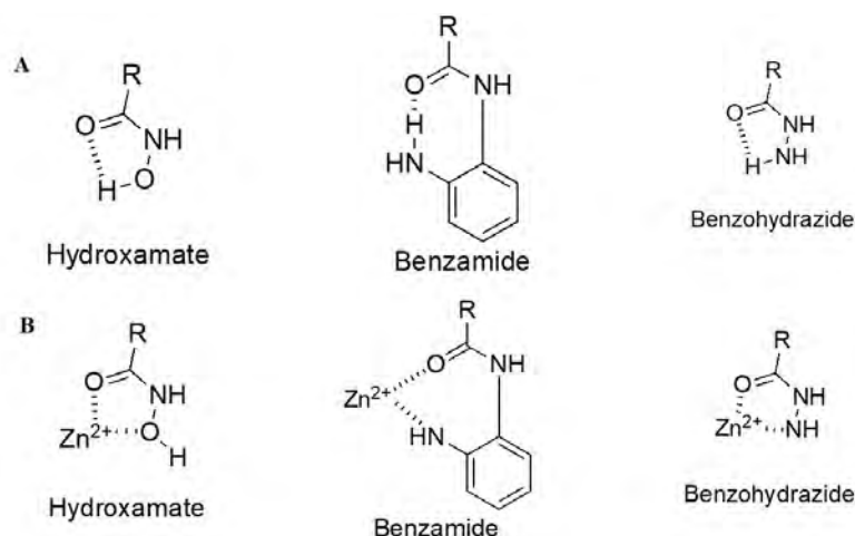
Figure 4. HDACi pharmacophore and chemotypes with juxtaposition to the critical Zn^{2+} ion. (A) Different chemotypes of ZBGs used to target class I HDACs with intramolecular hydrogen bonding patterns; (B) ZBGs coordinating to Zn^{2+}
