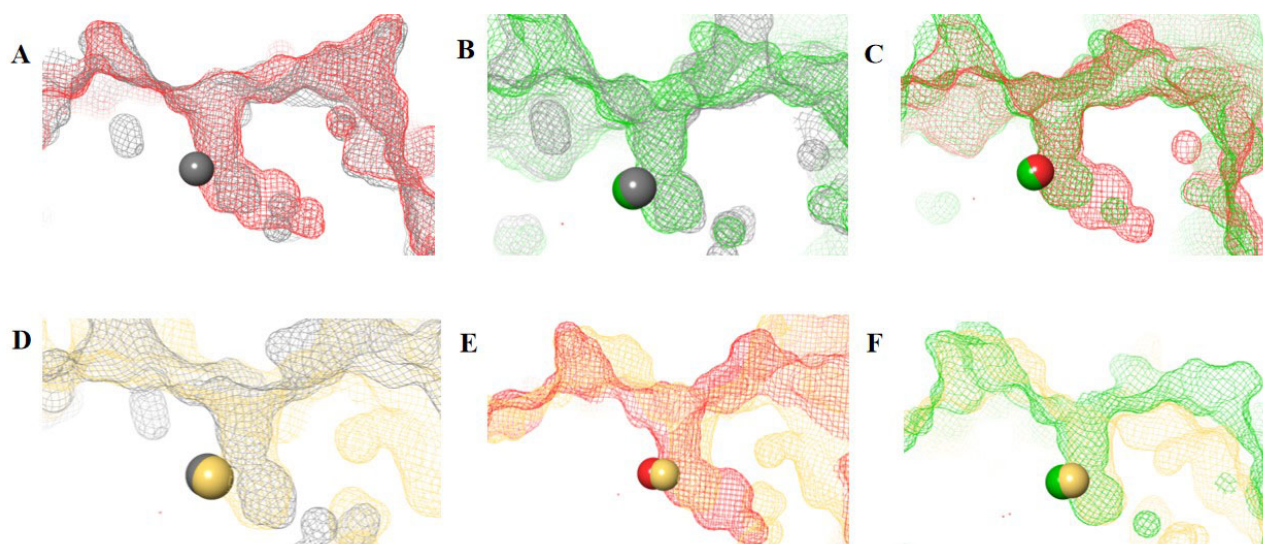
Figure 2. HDAC catalytic tunnel architecture. (A) Catalytic tunnels of HDAC1 (grey) and HDAC2 (red) superimposed; (B) catalytic tunnels of HDAC1 (grey) and HDAC3 (green) superimposed; (C) catalytic tunnels of HDAC2 (red) and HDAC3 (green) superimposed; (D) catalytic tunnels of HDAC1 (grey) and HDAC8 (gold) superimposed; (E) catalytic tunnels of HDAC2 (red) and HDAC8 (gold) superimposed; (F) catalytic tunnels of HDAC3 (red) and HDAC8 (gold) superimposed. Zn atoms are represented as spheres with the corresponding protein mesh surface colors. All images were generated via Maestro according to the PDB codes as detailed in Table 1
