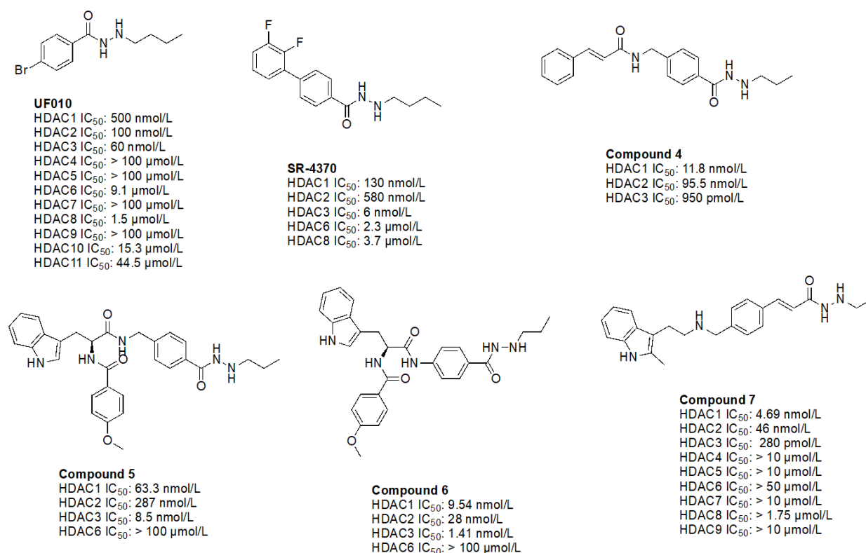
Figure 14. Examples of hydrazide HDACis [78–83]
