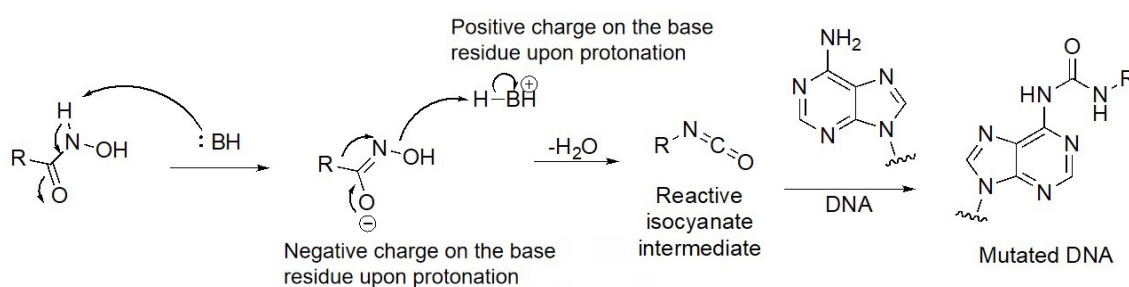
Figure 5. Lossen's rearrangement. The mechanism through a chemical reaction called Lossen's rearrangement is depicted, exemplified by a general hydroxamate through which the isocyanate intermediate forms, causing DNA mutagenesis and eventual toxicity [41]
