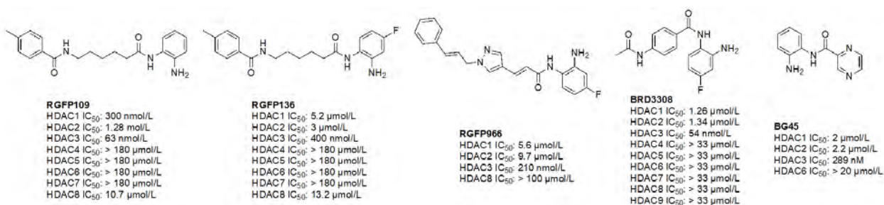
Figure 11. Examples of selective HDAC3 inhibitors [65–69]
