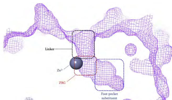
Figure 9. Structural presentation of the HDAC2 catalytic center. HDAC2 catalytic tunnel (PDB: 3MAX) labeled with HDACi binding moieties [58, 59]
