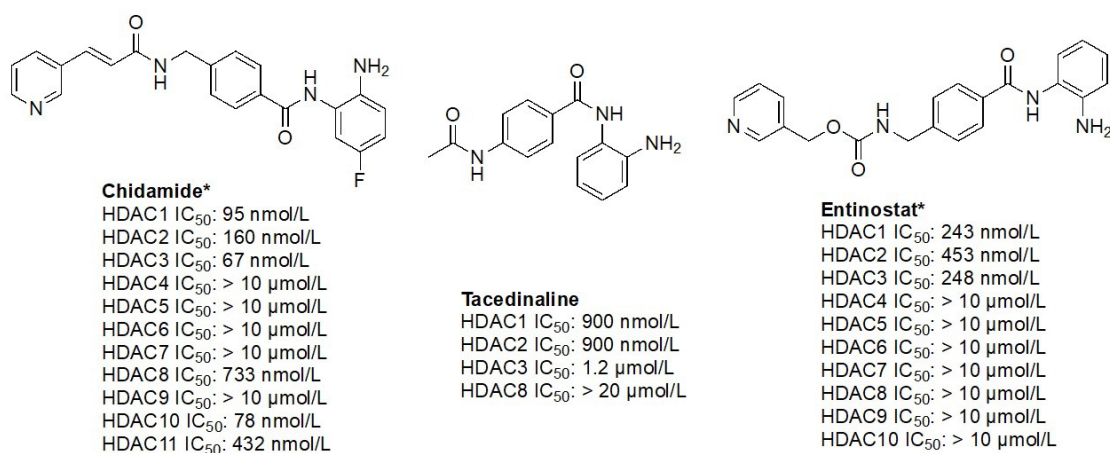
Figure 7. Examples of class I HDACi [55–57]. * Asterisks refer to inhibitors that are either clinical candidates or FDA-approved drugs
