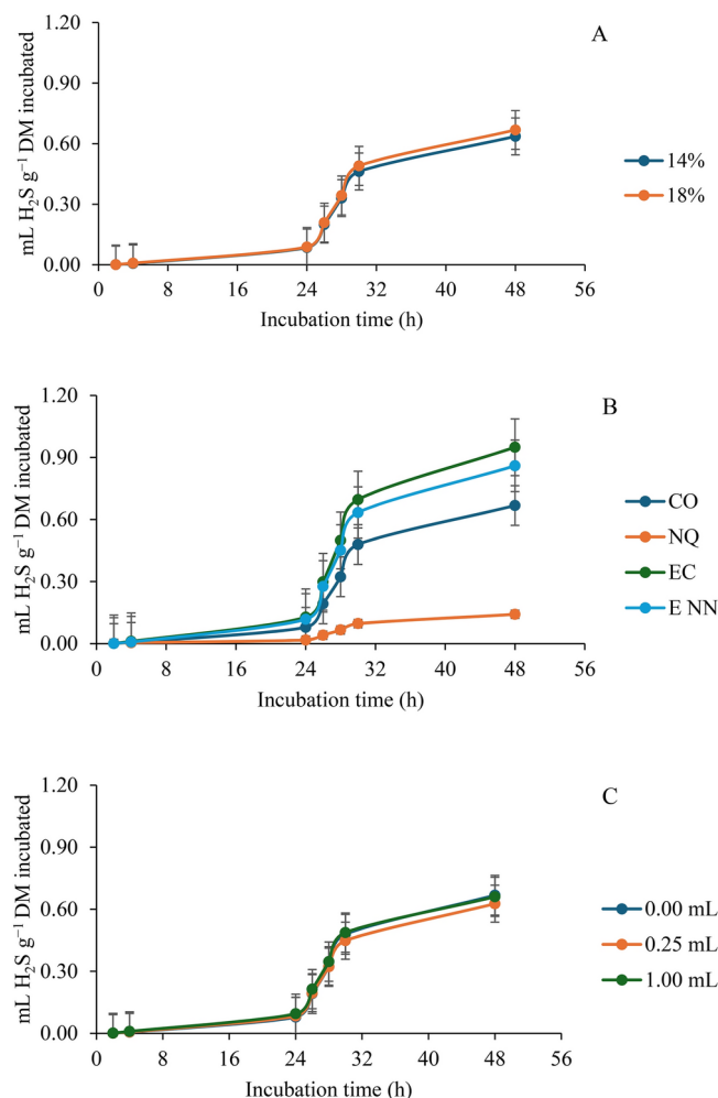
Fig. 5. Total hydrogen sulfide (H 2 S) production during in vitro rumen fermentation in response to (A) percentage of protein in the diet, (B) extract type, and (C) extract dose. The bars indicate the standard error of the mean. CO: Control; NQ: Nano-chitosan; EC: Crude extract; ENN: Nano-extract.
