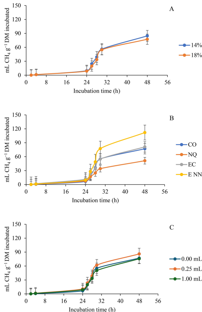
Fig. 3. Total methane ( \text{CH}_4 ) production during the in vitro ruminal fermentation response to (A) percentage of protein in the diet, (B) extract type, and (C) extract dose. The bars indicate the standard error of the mean. CO: Control; NQ: Nano-chitosan; EC: Crude extract; ENN: Nano-extract.
