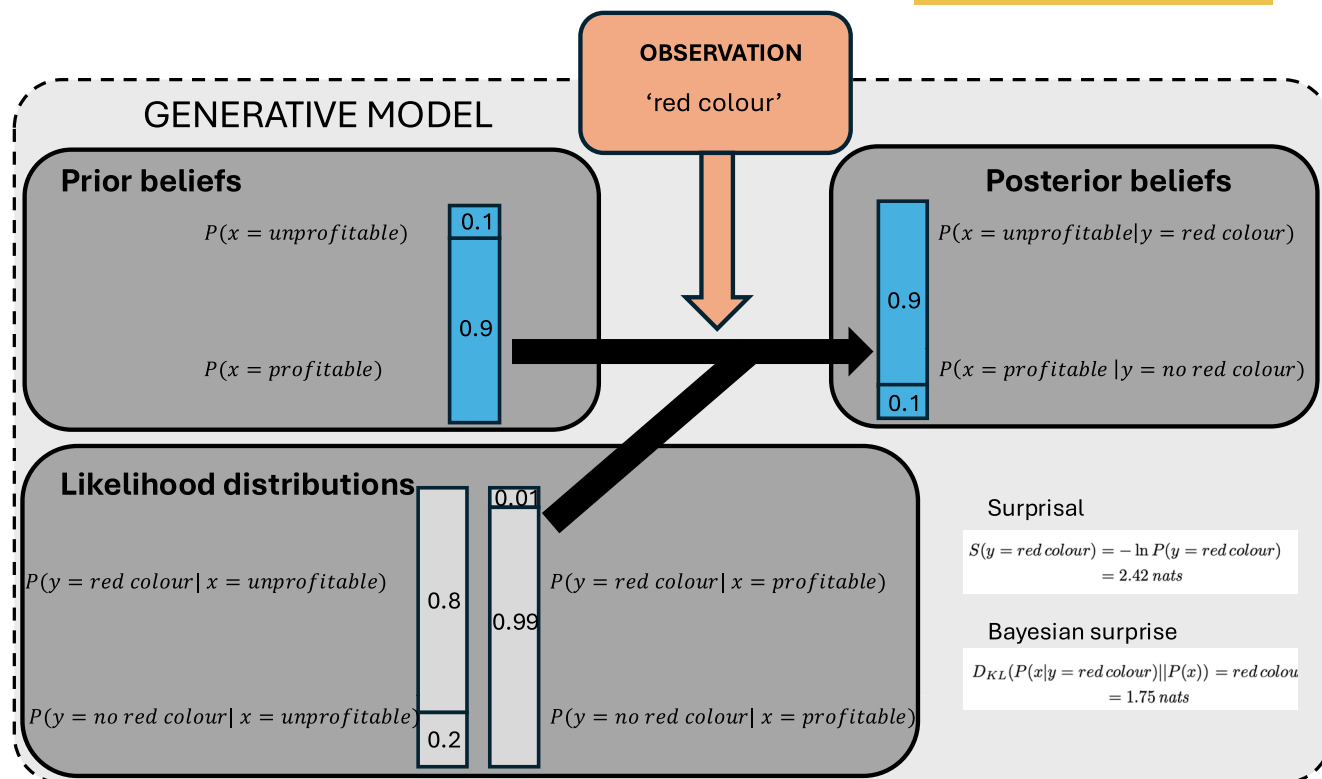
FIGURE 2 A simple generative model for Bayesian inference and active inference. Here we consider a space with two possible hidden states, x \in \{\text{'unprofitable', 'profitable'}\} and two possible observations y \in \{\text{'red colour', 'no red colour'}\} . The prior distribution gives the predator's prior belief about the possible state of an incoming prey, while the likelihood expresses how the predator probabilistically predicts what observation should be linked to what state (bar lengths not to scale). In Bayesian inference, once the predator sees the red colour ( y = \text{'red colour'} ) it can update its prior belief into its posterior belief. In active inference, the prior has a deeper meaning as it provides the organism's preferred states, which include its conditions for survival. In addition, active inference allows the organism to act so that its percepts match its preferences. Accordingly, when seeing the red colour, the predator may change its belief, by modifying its prior, or change its percepts, by moving away until encountering a prey that does not display the red colour (see Appendices S2 and S3 for the computation of surprisal and Bayesian surprise).
