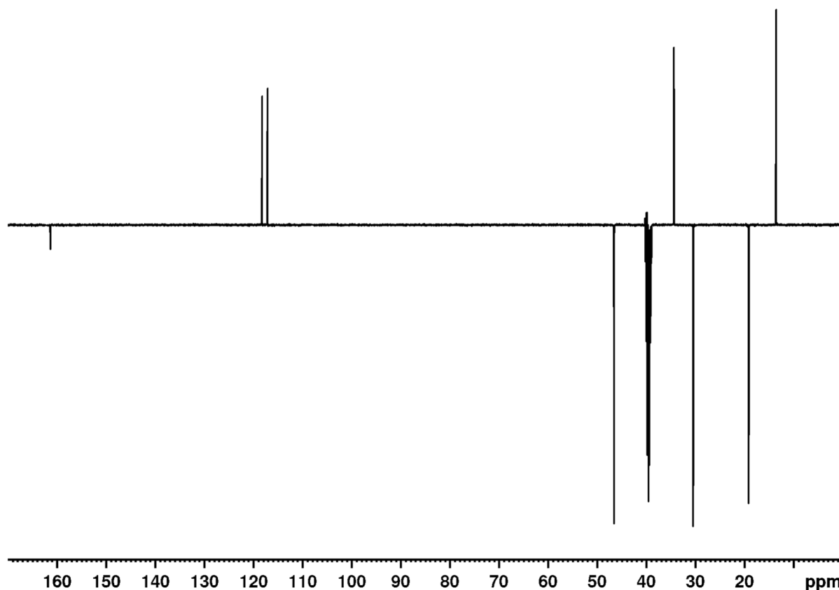
Fig. 2 13 C NMR spectrum of 1-butyl-3-methyl-1,3-dihydro-2 H -imidazole-2-thione ( 4 )
