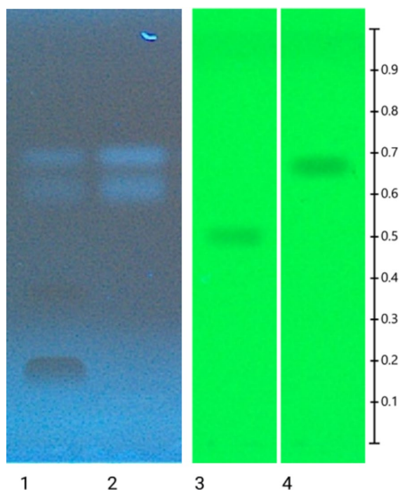
Fig. 8 HPTLC chromatograms of a model separation of equimolar mixtures of D-glucose and D-galactose containing 0.5% of EMIm-OAc (eluant: methanol/water, v/v=6/4). Track 1: direct measurement, track 2: measurement after IL removal through conversion into the corresponding thione by S_8 -treatment (separation conditions for monosaccharides). Tracks 3 and 4: HPTLC of thiones derived from EMIM and BMIM (separation conditions for thiones / treated samples)
