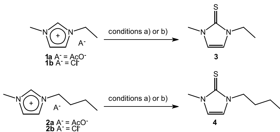
Scheme 1 Conversion of 1,3-dialkylimidazolium cations from ionic liquids into the corresponding 2-thiones by stirring with elemental sulfur. Conditions a preparative synthesis of an authentic sample according to a modified literature protocol (Laus et al. 2013), conditions b protocol for removing IL traces from analytical samples
