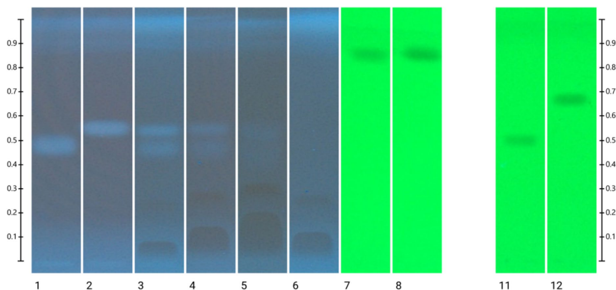
Fig. 5 HPTLC chromatograms of a model separation of equimolar mixtures of D-glucose and D-galactose. Track 1: 0.03 mg mL -1 D-glucose only; track 2: 0.03 mg mL -1 D-galactose only; Tracks 3–5: 0.03 mg mL -1 of each sugar, with 3) 0.2%, 4) 0.5% 5) 1% of EMIm-OAc ( 1a ); track 6: EMIm-OAc
