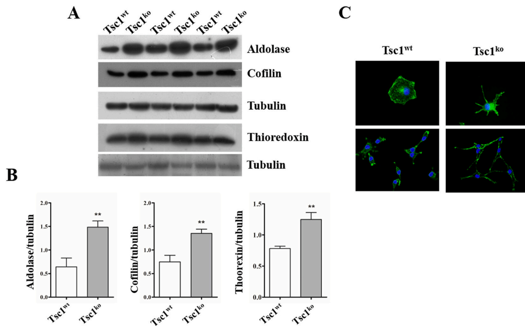
Fig. 5. Validation of proteomic results. A) Representative images of Western blotting experiments obtained using Ab against aldolase, cofilin, thioredoxin and tubulin; the latter was used as housekeeping protein. B) Bar graphs of results reported in panel A. Data represent the mean \pm SD. * p < 0.05 Tsc1 ko versus Tsc1 wt cells of three independent blots. C) Actin cytoskeleton analysis by fluorescent phalloidin, scale bar = 50 \mu m.
