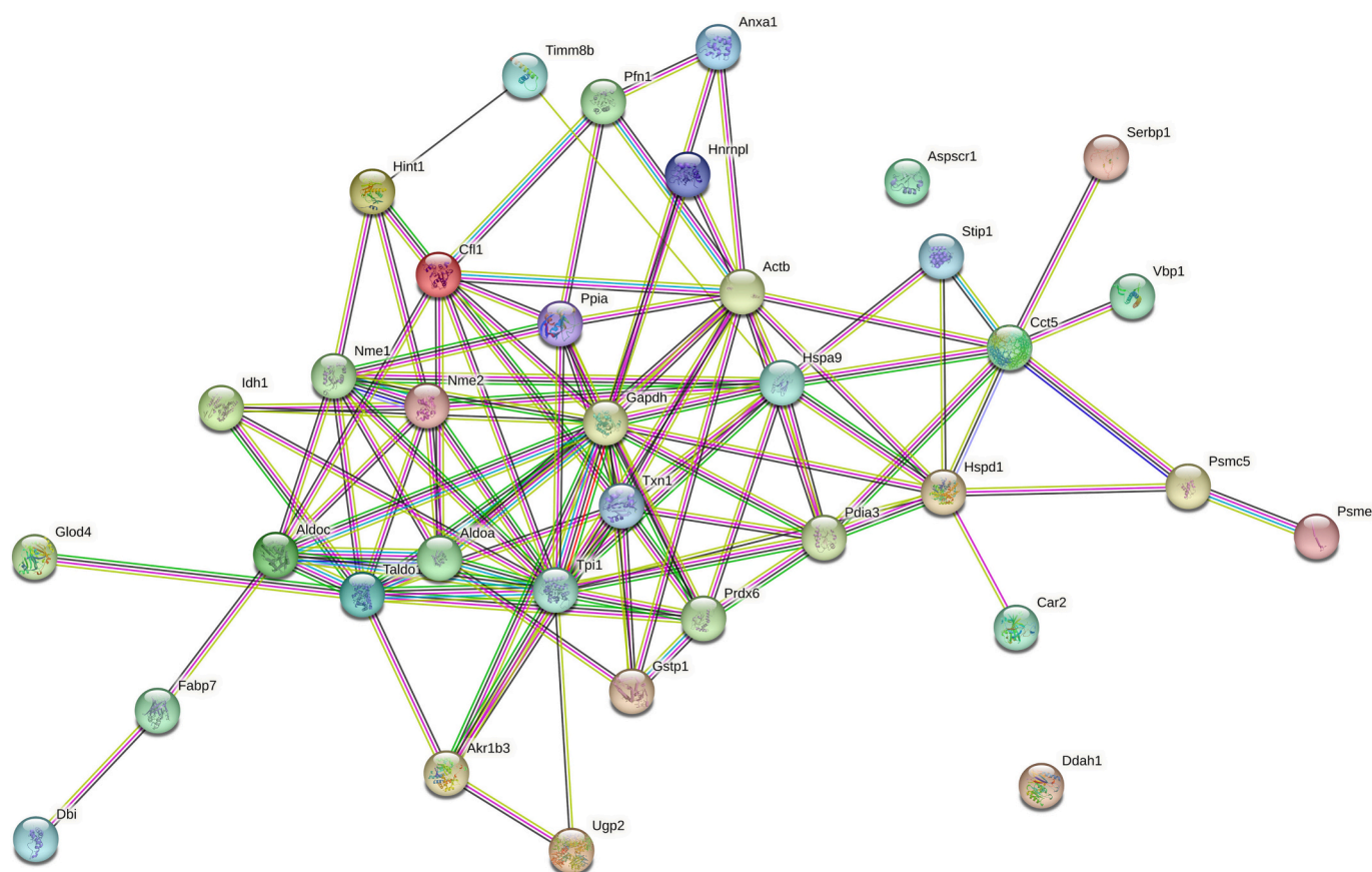
Fig. 3. Protein-protein interaction (PPI) of differentially abundant proteins in Tsc1^{ko} versus Tsc1^{wt} cells (PPI enrichment p -value: <1.0 \times 10^{-16} ) after STRING analysis. Functional protein association network of proteins listed in Table 1, as deriving from a database search in STRING. Gene name of proteins are reported, for full names see Table 1.
