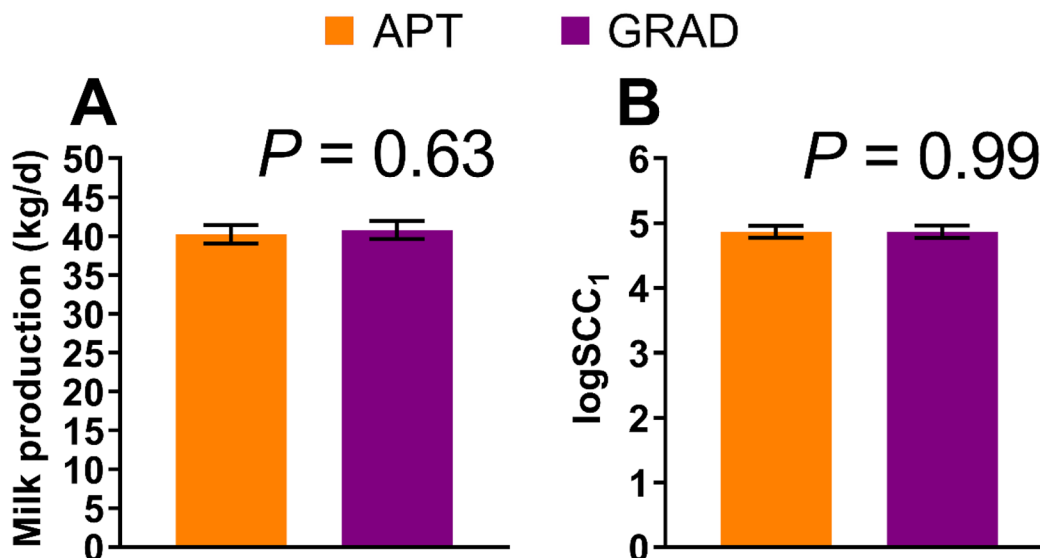
Figure 5. Least squares means from general linear models showing the effect of gradual cessation of milking (GRAD) versus abrupt cessation of milking (APT) at the end of lactation on milk production at the first test date after calving (A) and the SCC ( \log_{10} -transformed, \log\text{SCC}_1 ; B) at the first test date after calving. Cows in the APT group were milked 3 times daily until the day of dry-off, whereas cows in the GRAD group were milked once daily for 7 d before dry-off. Error bars show 95% CI.
