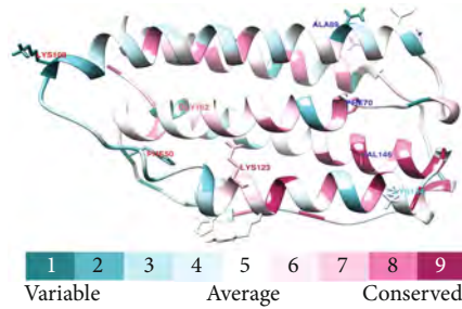
FIGURE 3: The conserved Ig domain of IFNε was found by pinpointing amino acid locations that were favorably chosen. For this, we utilized the Phyre tool ( http://www.sbg.bio.ic.ac.uk/phyre2/html ) to draw positively selected regions onto the crystal structure of the IFN protein from M. javanica , which served as a reference sequence. The INFab domain, which contains the ligand-binding site, contains the residues that have been selected. These include a cluster of sites immediately following the signal sequence and the ligand-binding site region. The precise localization of favorably chosen amino acid sites in IFN proteins. With conservation values ranging from 1 to 9, we were able to make educated guesses about which amino acids will be conserved. Conservation values of 1-4 are considered variable, 5-6 show average conservation, and 7-9 indicate very high conservation.
