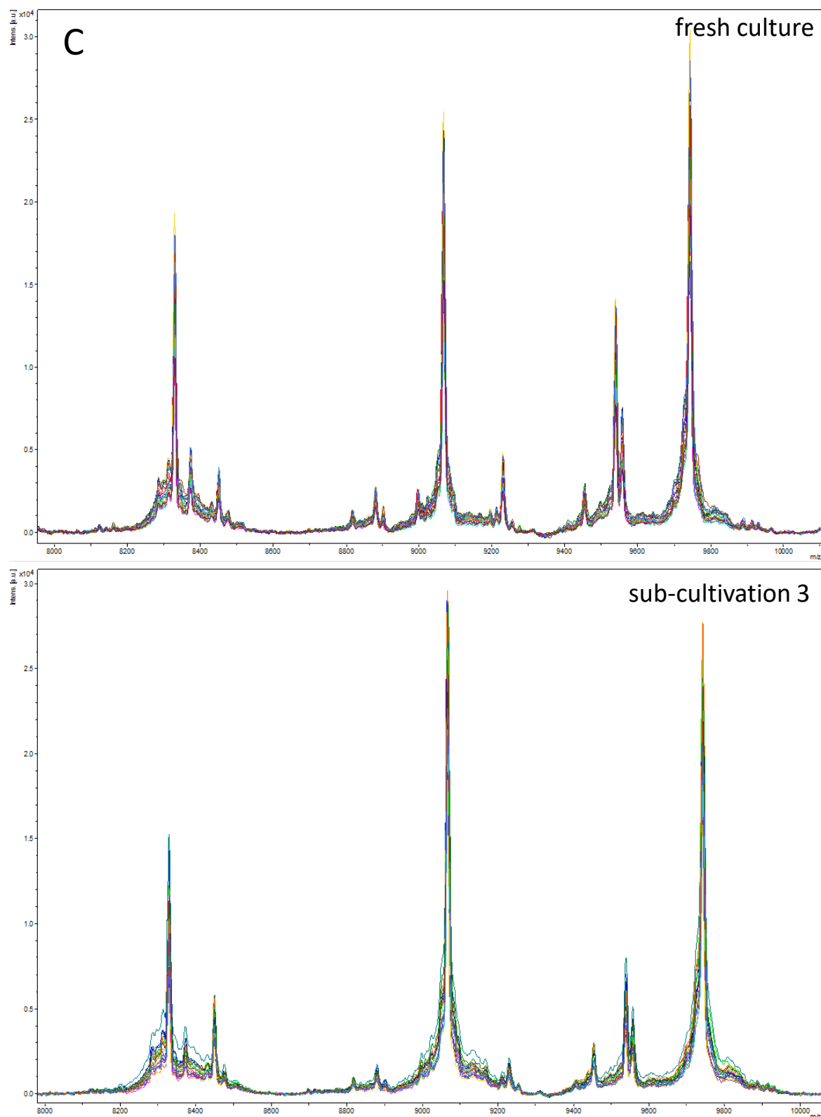
Figure 2. Influence of sub-cultivation (fresh culture vs. sub-cultivation step 3) on spectra quality with a decrease of peak intensity. Shown for E. coli isolate 16/1523-3 KnoRe 2 ( n = 20 spectra). (A) Within the range of 4000–6000 m/z ; (B) Within the range of 6000–8000 m/z ; (C) Within the range of 8000–10000 m/z .
