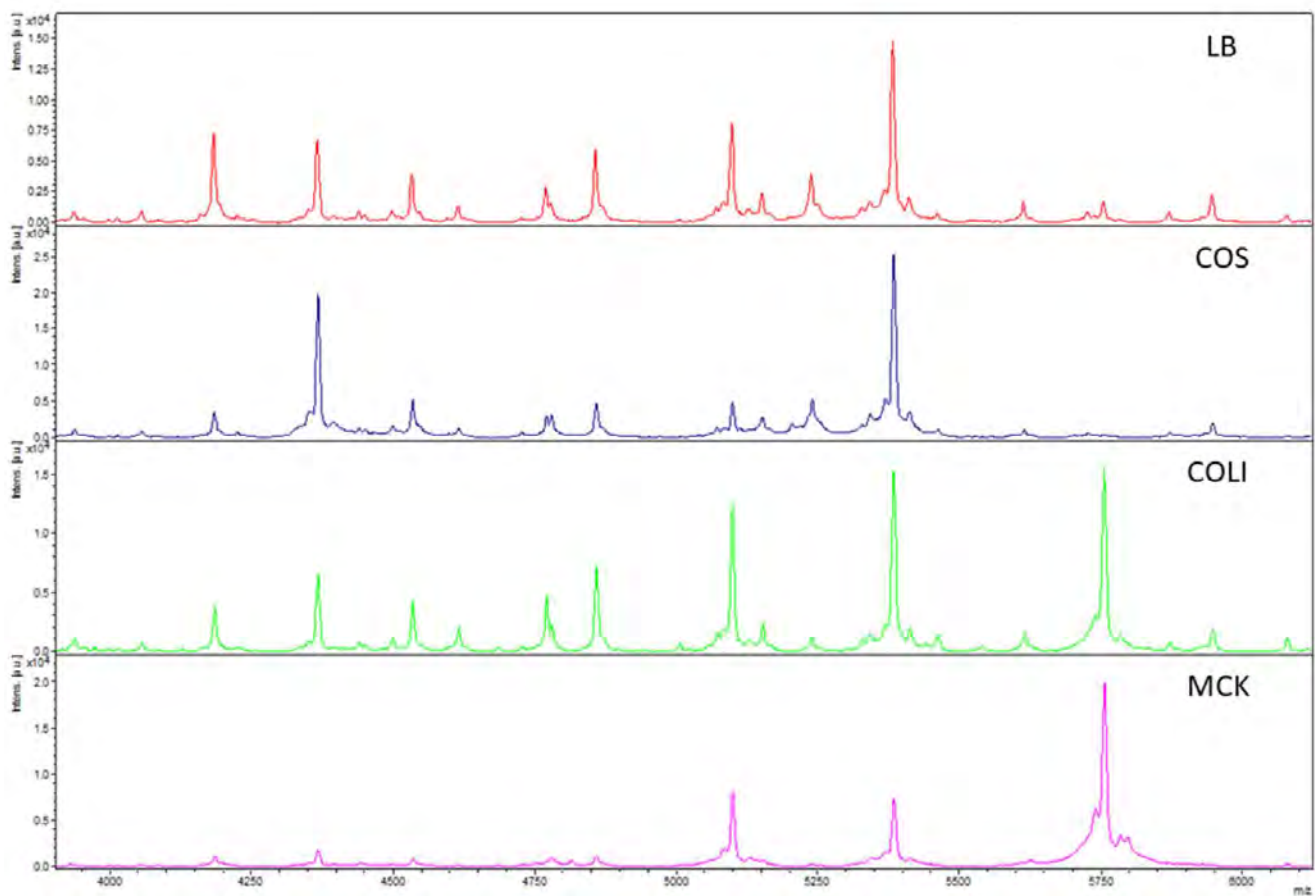
Figure 1. Reproducibility of spectra on different solid agars shown for E. coli isolate 16/01363-1 (LB: Luria Broth agar; COS: Columbia agar with sheep blood; COLI: Coliformen agar; MCK: MacConkey agar). Differences in intensity and quantity of peaks are shown within the range of 4000–6000 m/z .
