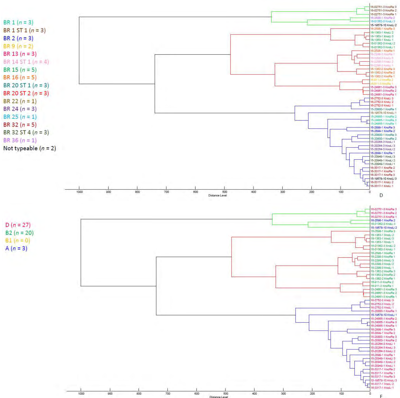
Figure 5. Clustering of 50 randomly selected E. coli isolates from eight farms based on their farm origin (A), the presence of femoral head necrosis (B), their serotype (C), their PFGE profile (D), and their phylogroup (E).
