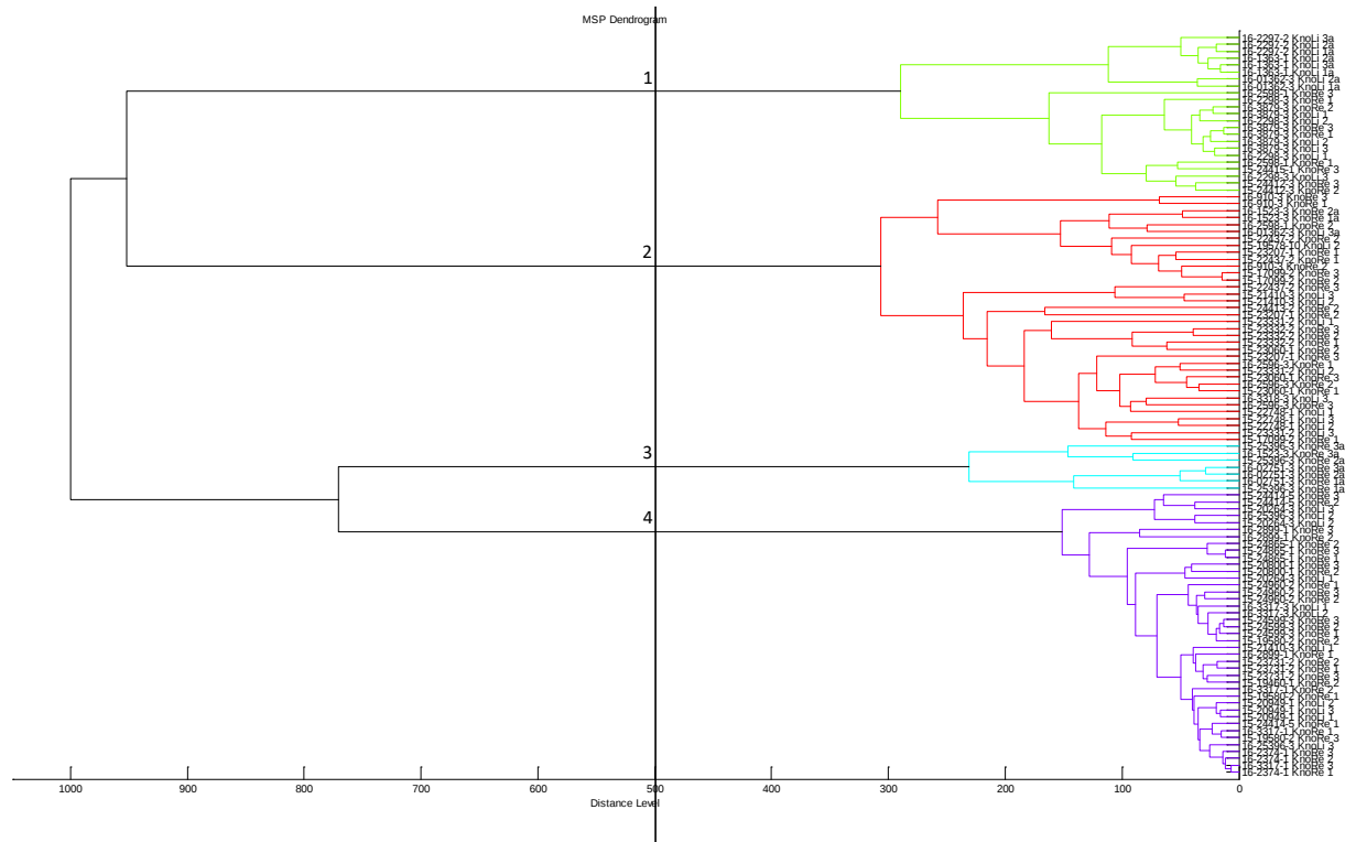
Figure 4. Score oriented MSP dendrogram based on 107 E. coli isolates revealing four distinct clusters (distance level 500).
