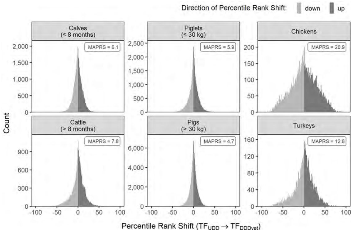
FIGURE 4 | Shift in percentile ranks if farms were ranked by DDDvet-based treatment frequencies ( TF_{DDvet} ) instead of UDD-based treatment frequencies ( TF_{UDD} ) for each of the six animal populations covered by the German benchmarking system. Note that the count axis in each panel is scaled individually. Data is from all half-year periods 2014-2 to 2017-2. MAPRS, median absolute percentile rank shift.
