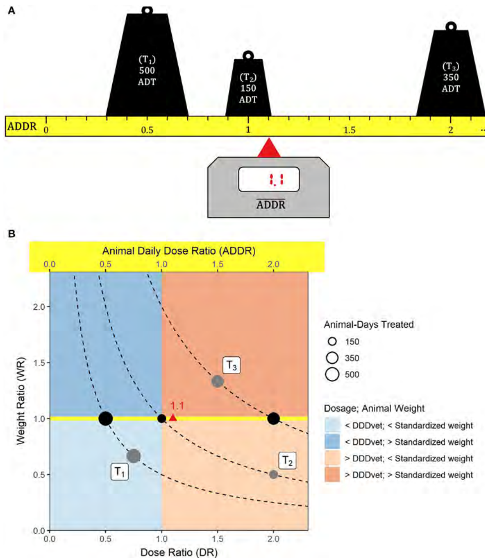
FIGURE 1 | An example illustrating the average animal daily dose ratio. Three treatments take place on a farm: (T 1 ) 500 animal-days treated (ADT) with an animal daily dose ratio (ADDR) of 0.5, (T 2 ) ADT = 150, ADDR = 1 and (T 3 ) ADT = 350, ADDR = 2. (A) Each treatment is represented by a weight according to the number of animal-days treated that is located on a ruler measuring the animal daily dose ratio on a linear scale (the ruler is assumed to be weightless and may extend further to the right if necessary). The average animal daily dose ratio ( \overline{\text{ADDR}} = 1.1 ) marks the point of support on the ruler where the setup balances out. (B) The treatments are shown as gray circles on a Cartesian plane where the abscissa of the circle's center is the dose ratio, its ordinate is the weight ratio, and where the area of the circle represents the number of animal-days treated. Each treatment is located on a hyperbole (dashed curves) along which the ADDR is constant. Therefore, in terms of the animal daily dose ratio the black circles are equivalent to the original treatments T 1 , T 2 , and T 3 . They are located on a yellow strip that is equivalent to the ADDR ruler in (A) and whose values can be read off the upper abscissa. The red triangle marks the \overline{\text{ADDR}} value.
