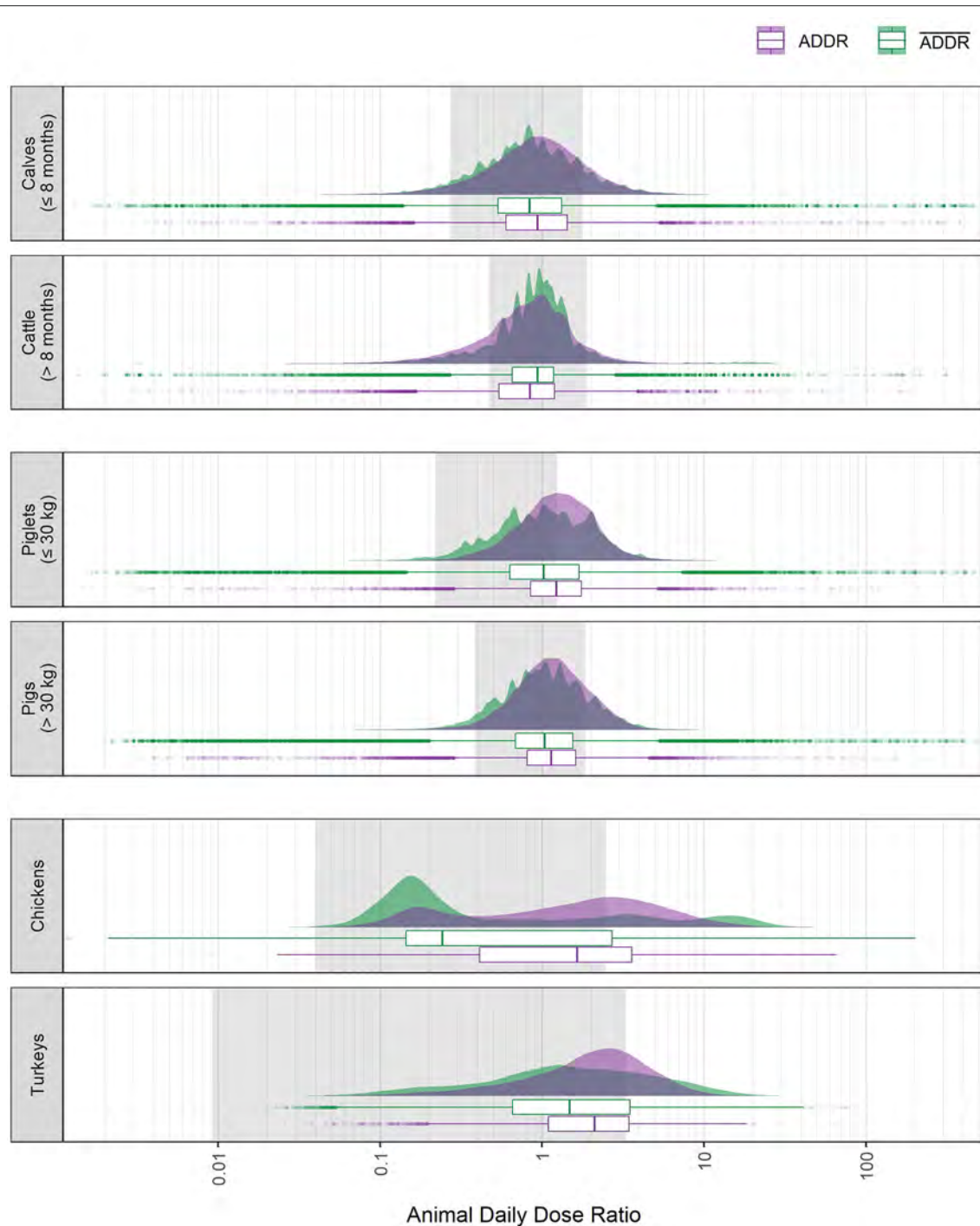
FIGURE 5 | Distribution of the animal daily dose ratio at the individual treatment level (ADDR, purple) and at the farm level (ADDR, green) for each of the six animal populations covered by the German benchmarking system. The regions shaded in gray indicate the weight ratio range for each of the animal populations (compare Table 1). The abscissa is log-scaled. Data is from all half-year periods 2014-2 to 2017-2.
