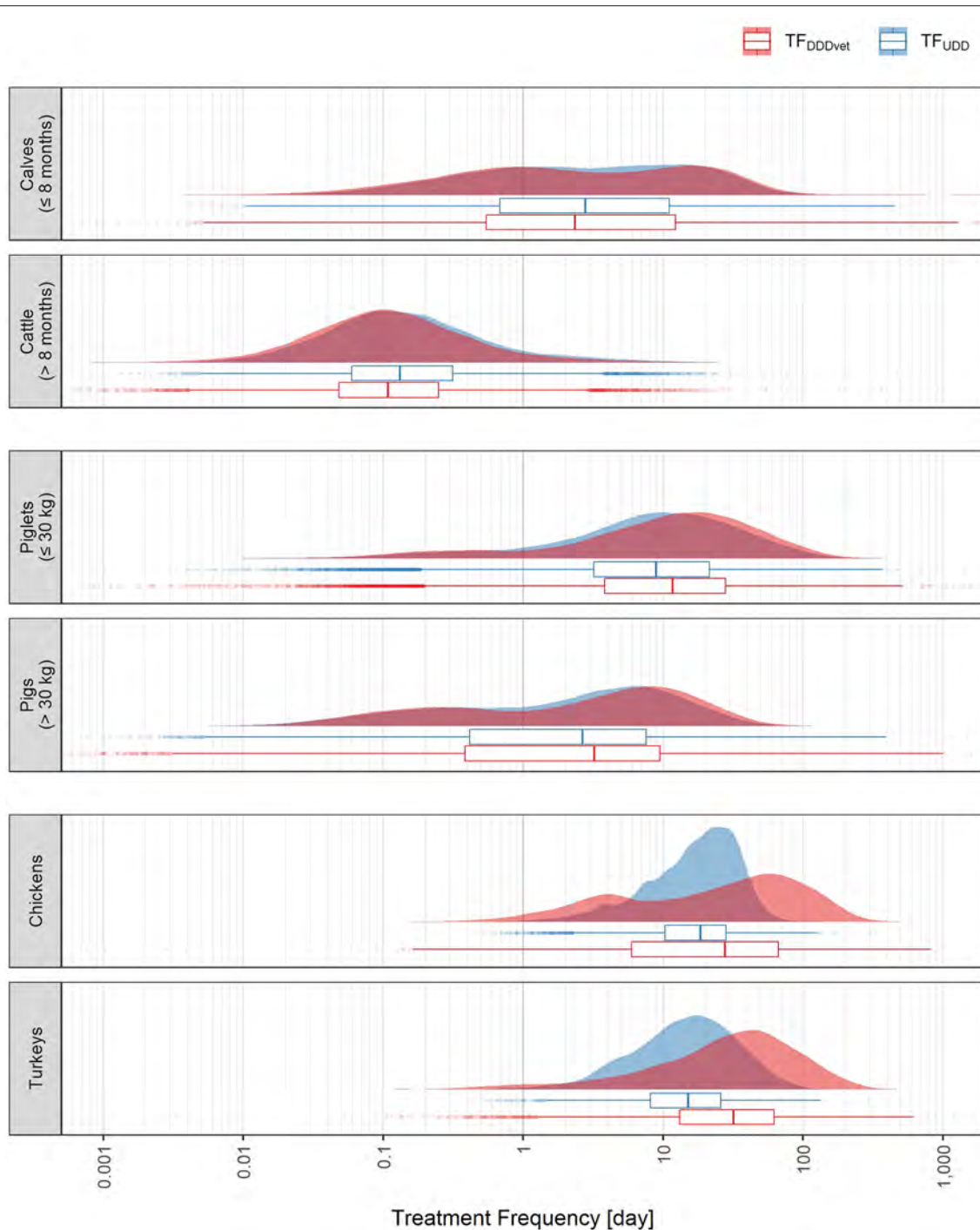
FIGURE 3 | Distributions of UDD-based treatment frequencies, TF_{UDD} (blue), and DDDvet-based treatment frequencies, TF_{DDDvet} (red), for each of the six animal populations covered by the German benchmarking system. The abscissa is log-scaled. Data is from all half-year periods 2014-2 to 2017-2.
